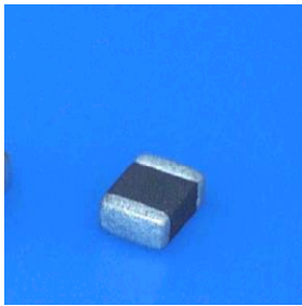
MIPSAZ2520DxxFH series (2.5 x 2.0 x 1.2mm max)
